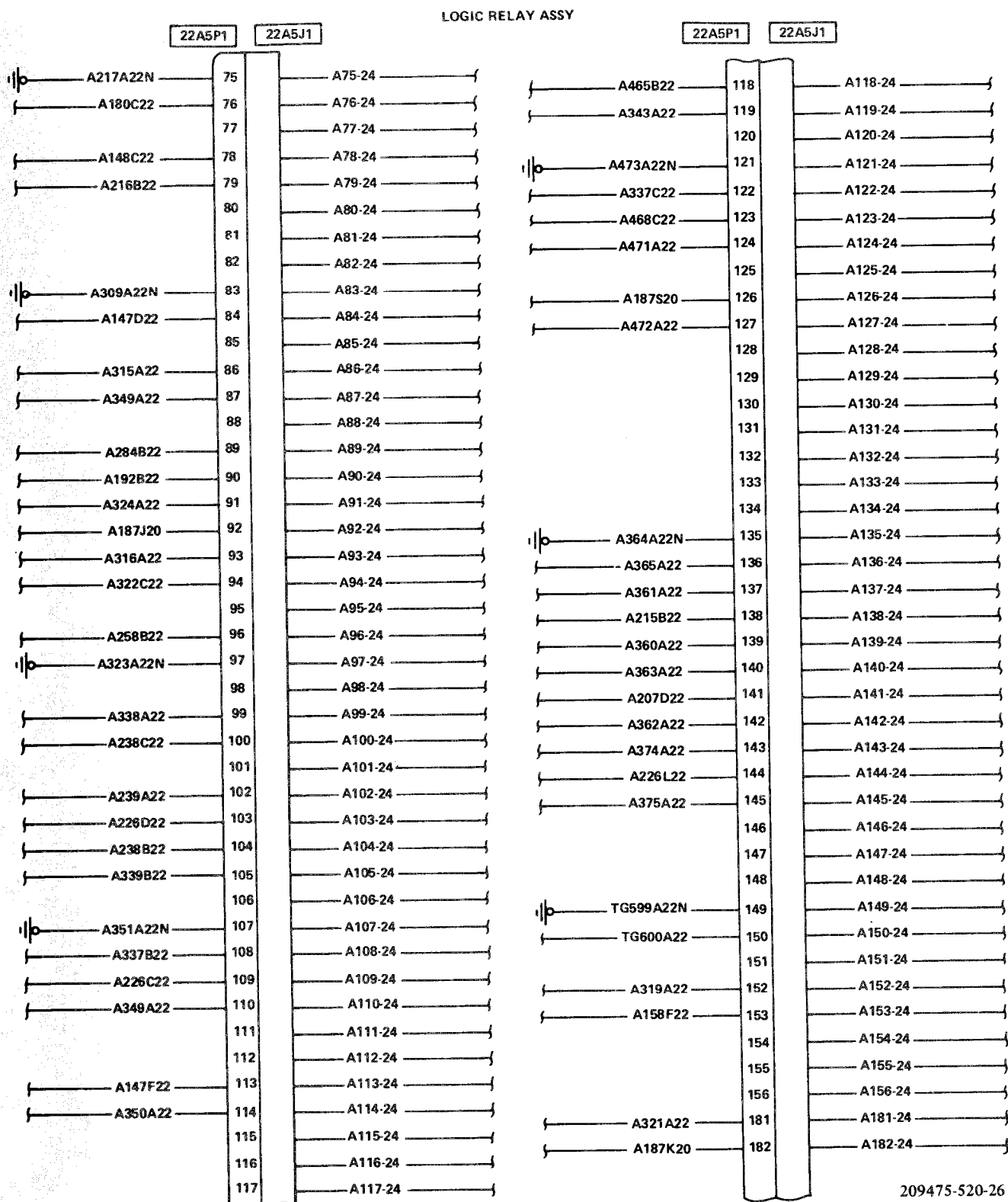
Figure F-76. M Electrical Equipment Component Replacement (Sheet 20 of 38)
