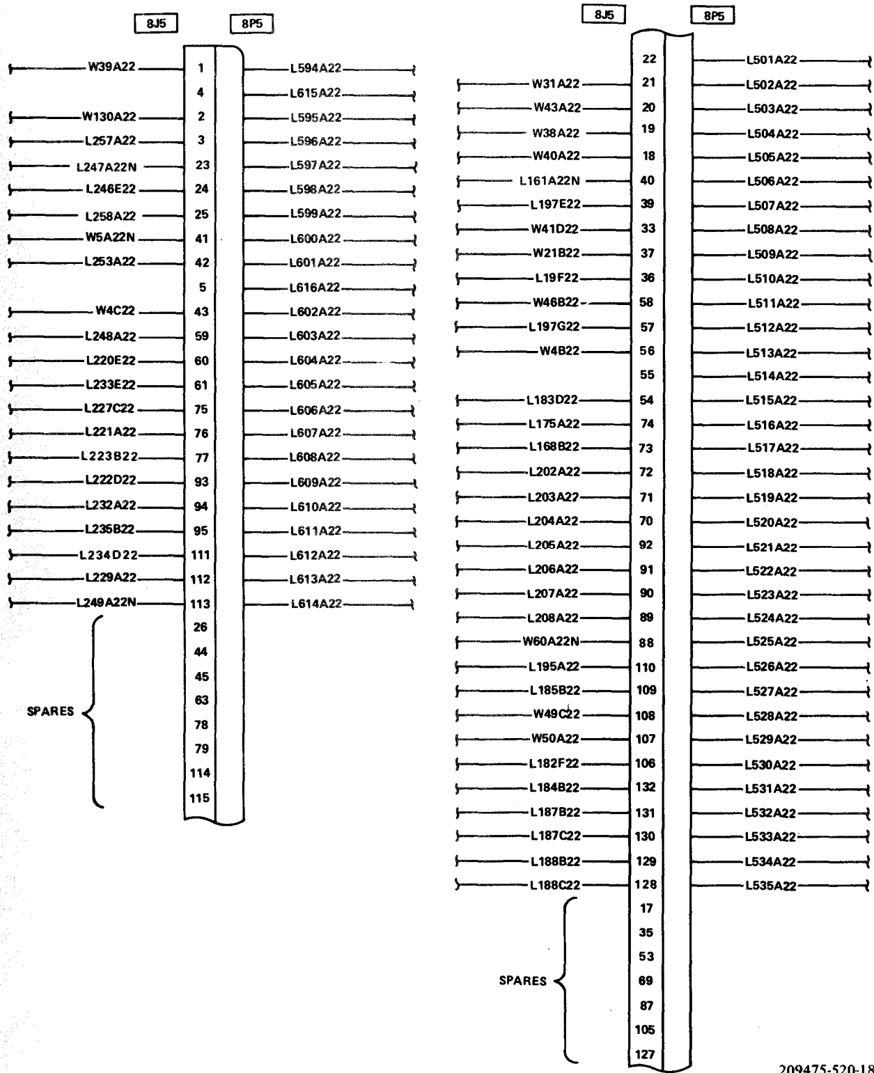
Figure F-76. M Electrical Equipment Component Replacement (Sheet 12 of 38)
