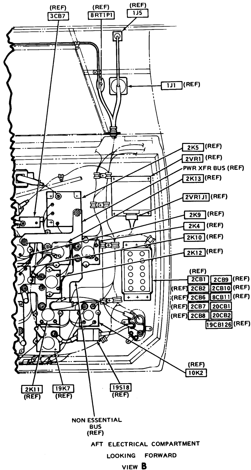
Figure F-73. M TOW Missile Armament Subsystem (Equipment Location) (Sheet 3 of 16)
