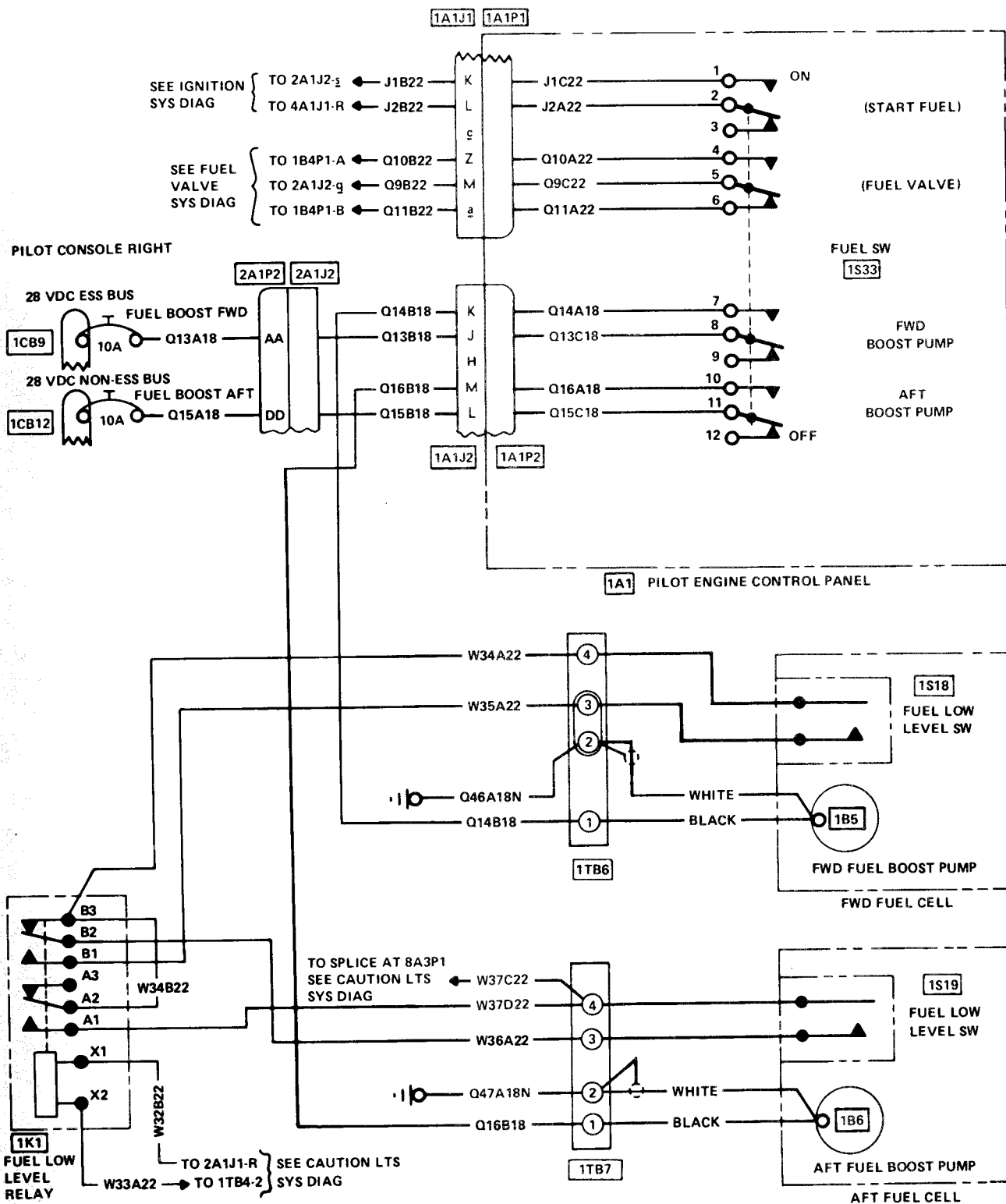
Figure F-9. P Fuel Boost System Wiring Diagram
