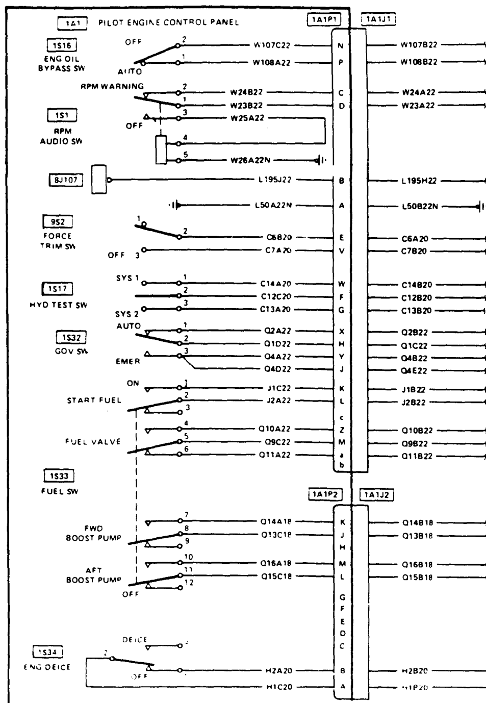
Figure F-76. M Electrical Equipment Component Replacement (Sheet 1 of 38)
