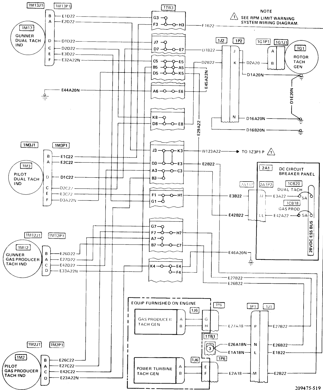
Figure F-41. M Tachometer Indicating Systems (Sheet 1 of 10)
