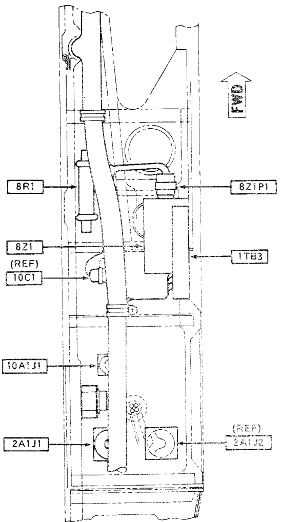
PILOT STATION RH SIDE LOOKING UP DETAIL B
