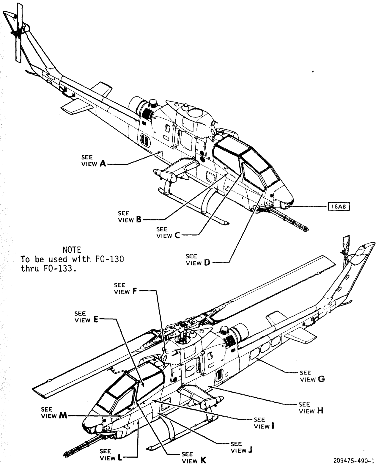
Figure F-74. Fire Control System (Equipment Location) (Sheet 1 of 14)
