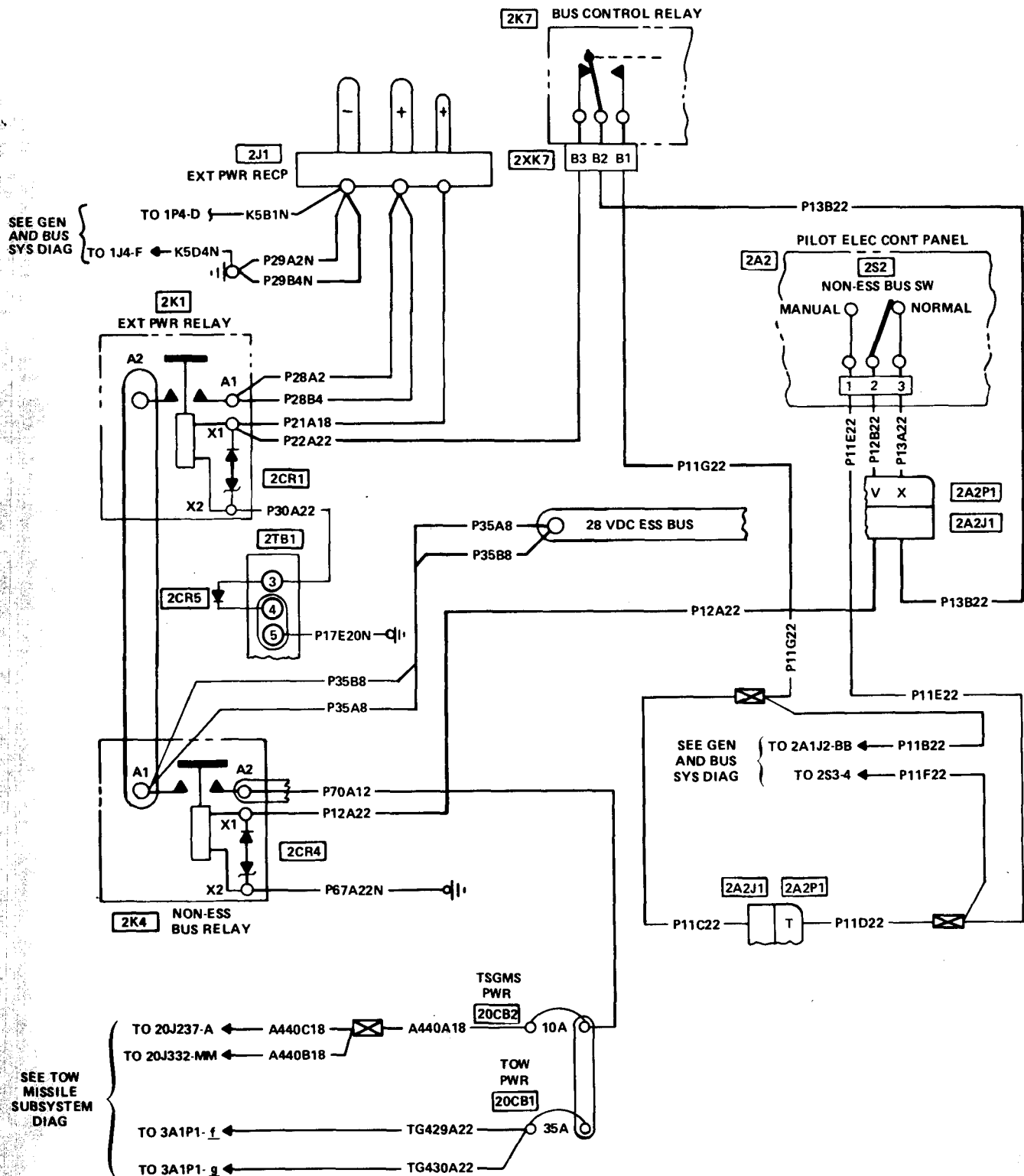
Figure F-2. p External Power System Wiring Diagram
