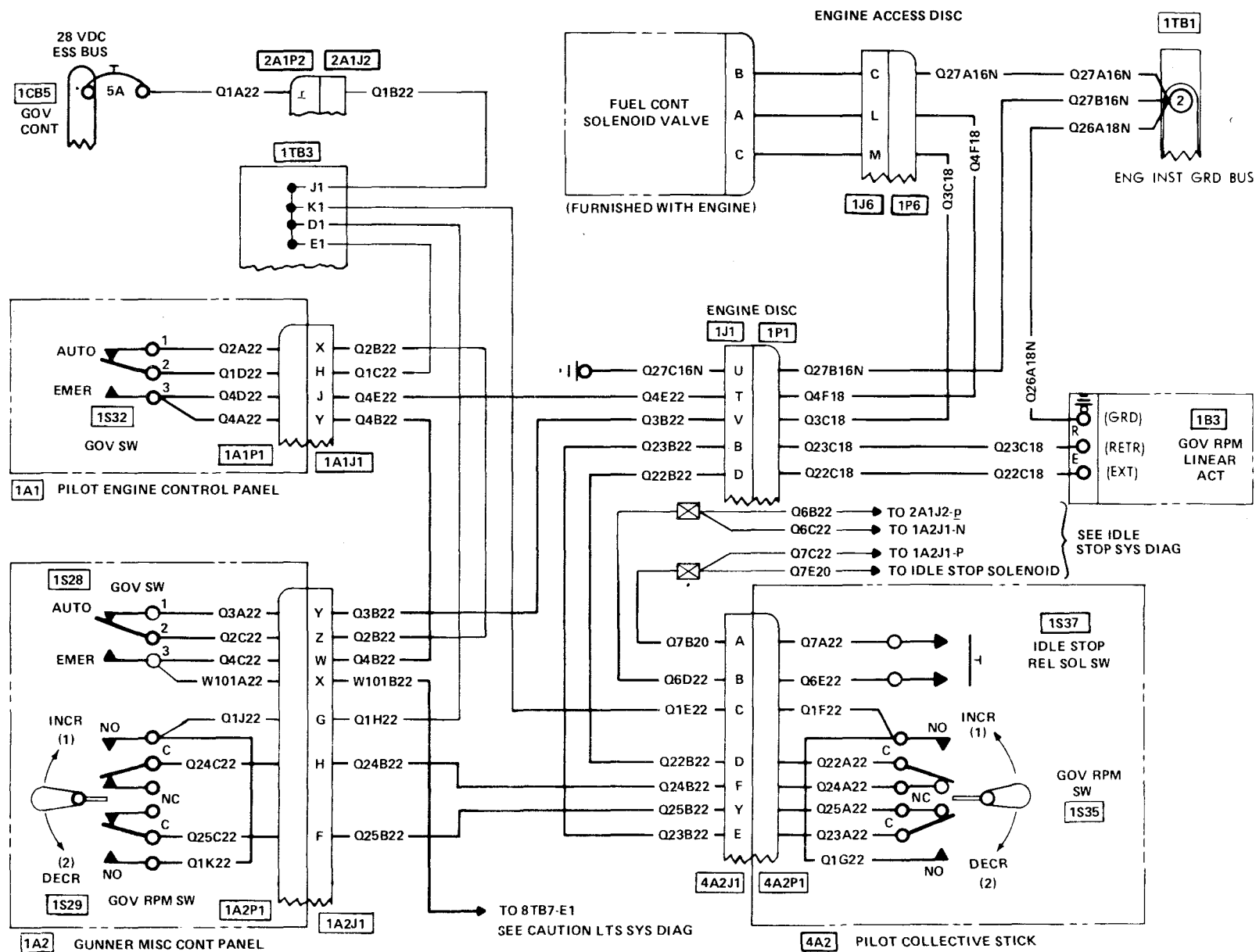
Figure F-10. Governor Control System Wiring Diagram
