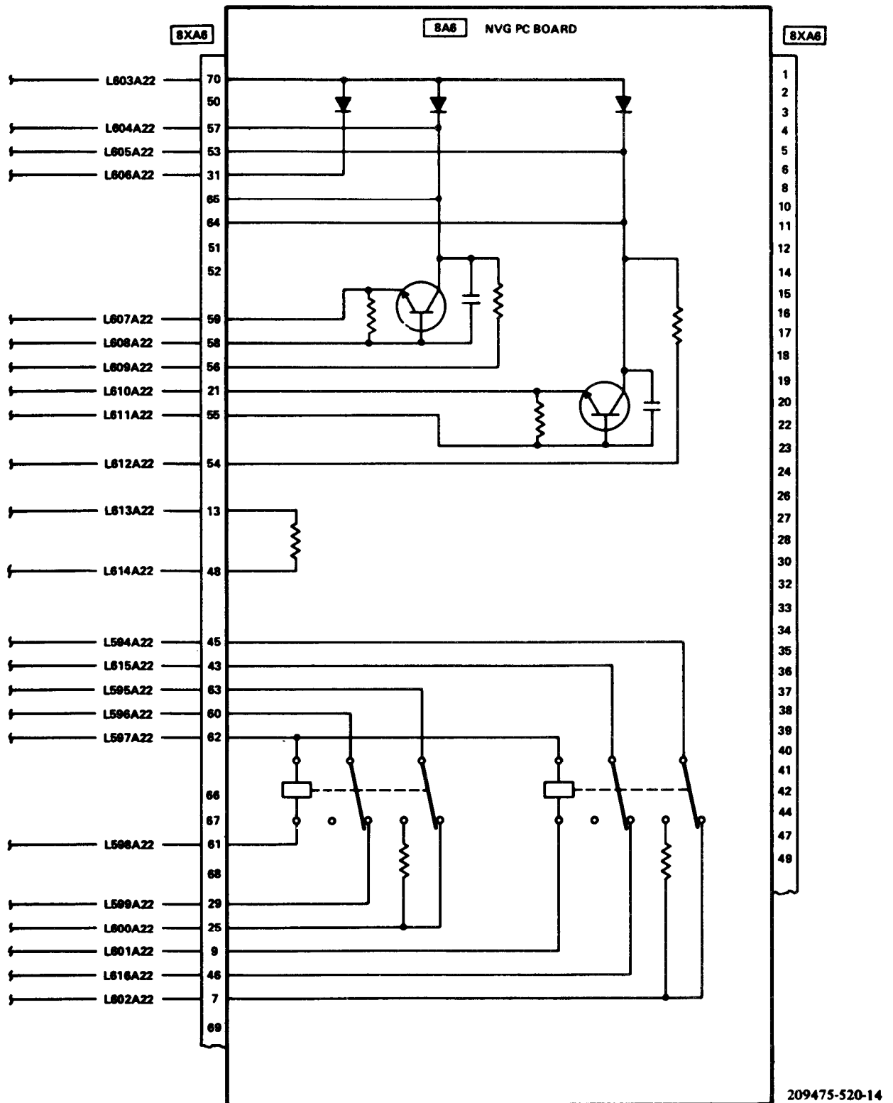
Figure F-76. Electrical Equipment Component Replacement (Sheet 8 of 38)
