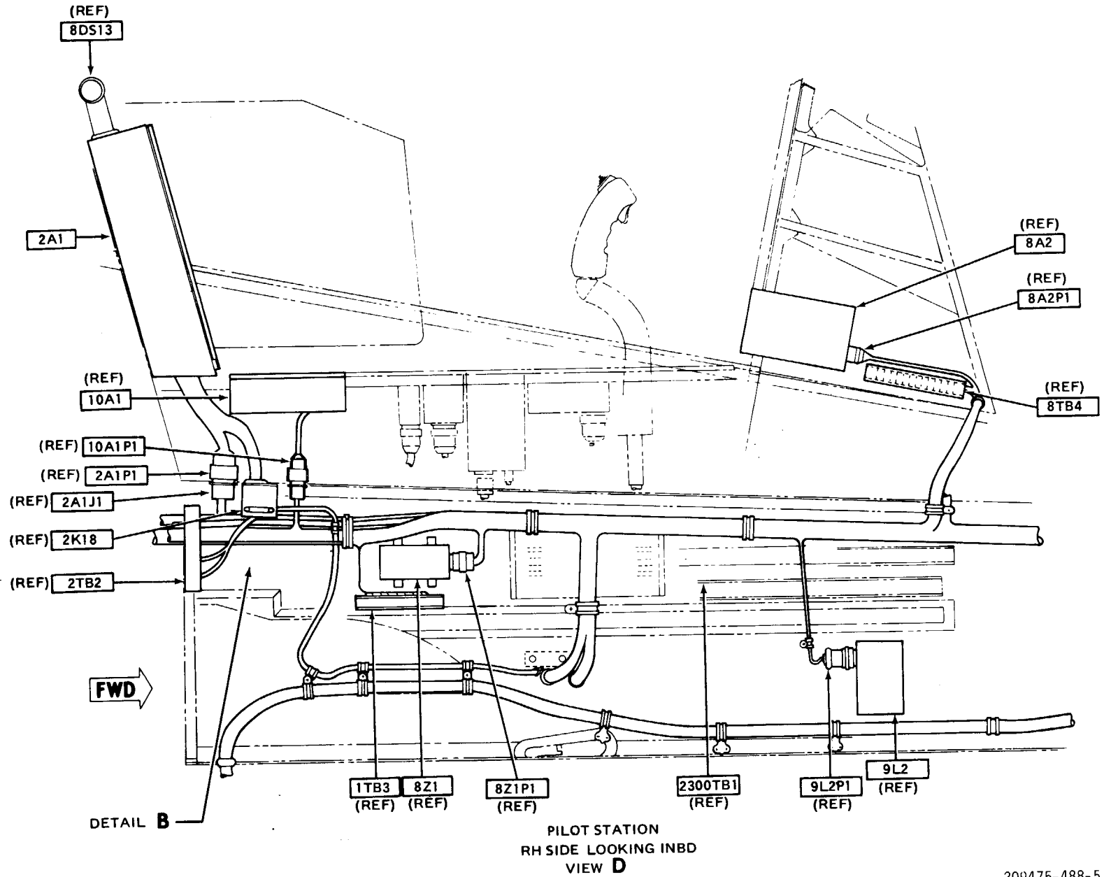
Figure F-52. M AC Power System (Equipment Location) (Sheet 5 of 10)
