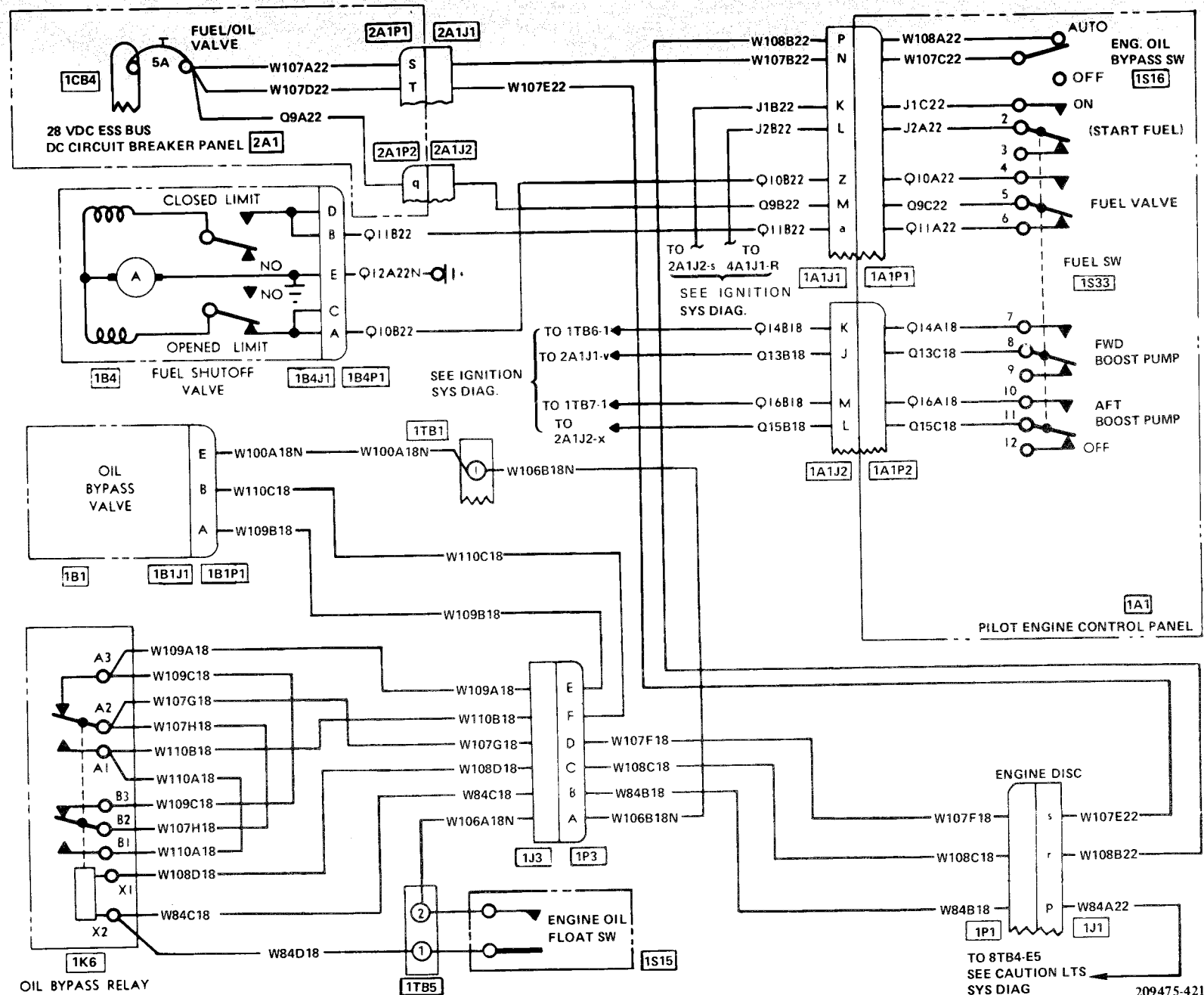
Fuel Valve and Engine Oil Valve System Wiring Diagram
