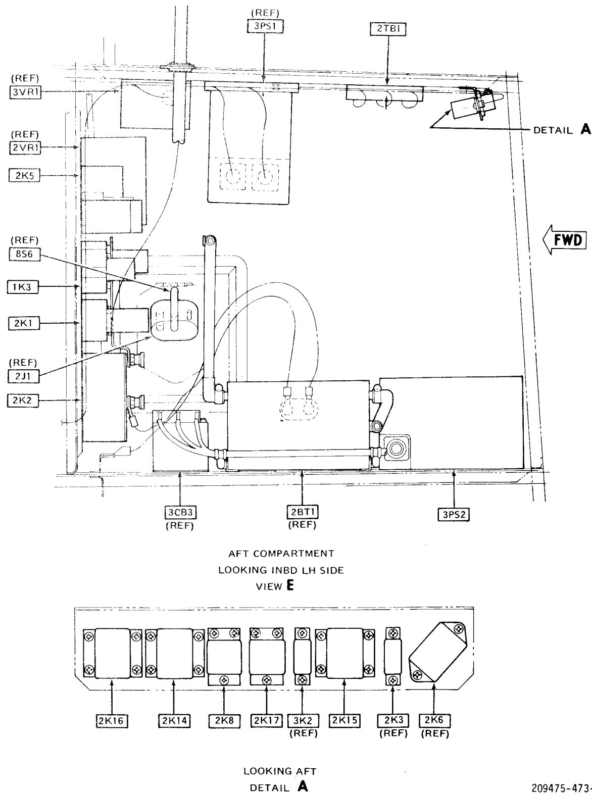
Figure F-51. M DC Power Distribution and Interconnect Logic (Equipment Location) (sheet 6 of 7)
