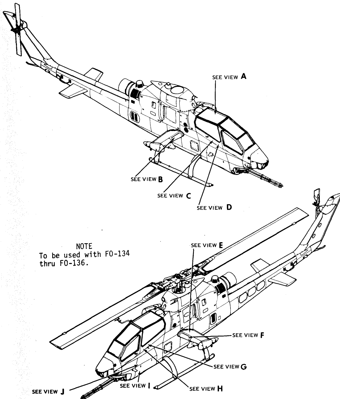
Figure F-75. Wing Stores Armament Subsystem (Equipment Location) (Sheet 1 of 12)
